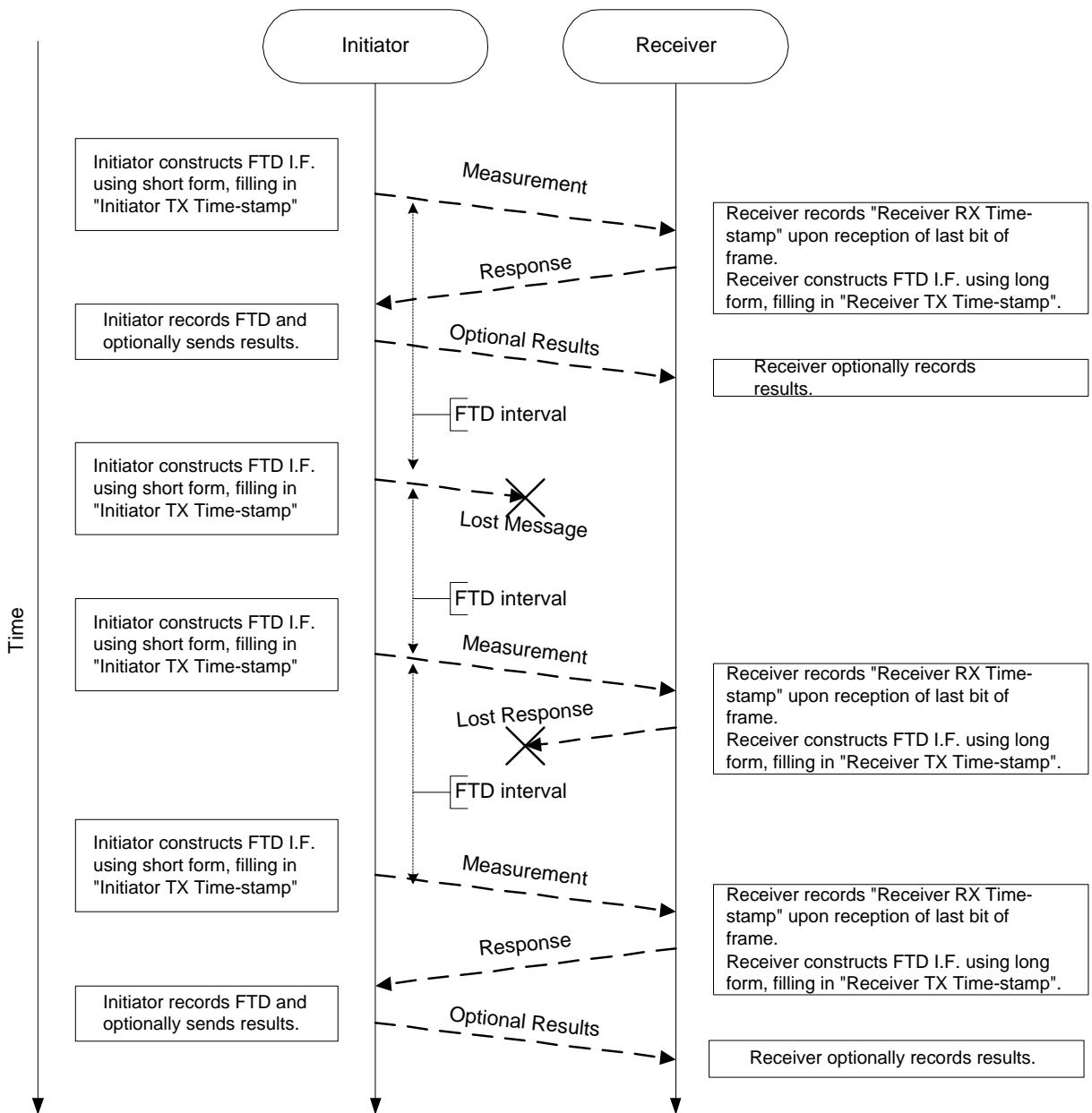
Figure B - 2 - Frame Transfer Delay Measurement
